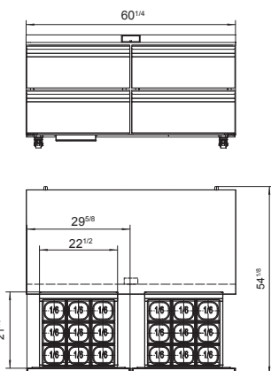
Casters
